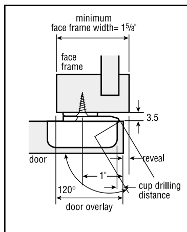
TEC 830 with wrap around baseplate
