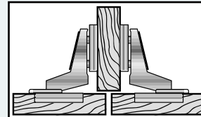
Half Overlay
