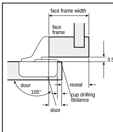
TEC 831 with side mount baseplate
