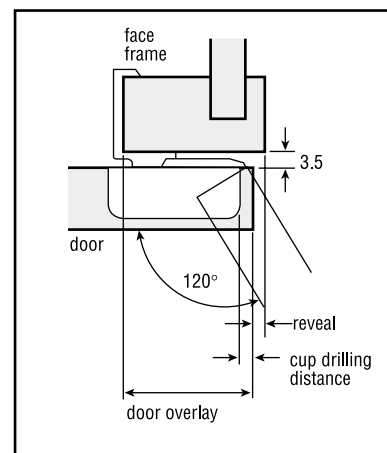
TEC 830 with face mount baseplate
